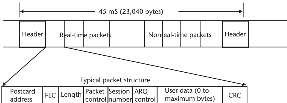
Figure 9.15 Outbound packetized TDM time frame (typical).
